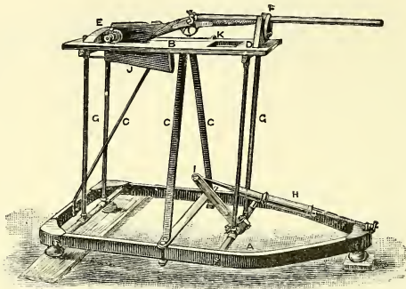
New Mechanical Gun-Rest and Recoil-Gauge.
